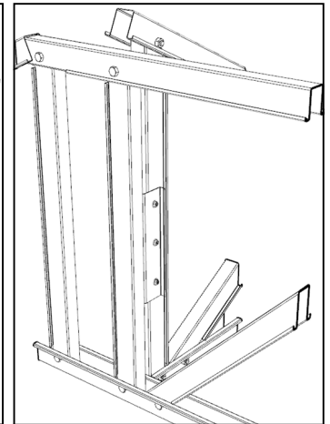
250 x 0.95mm Truss Profile fixed with Tek screws required for the load
