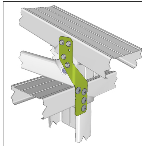
Typical C Section Truss Hold Down
