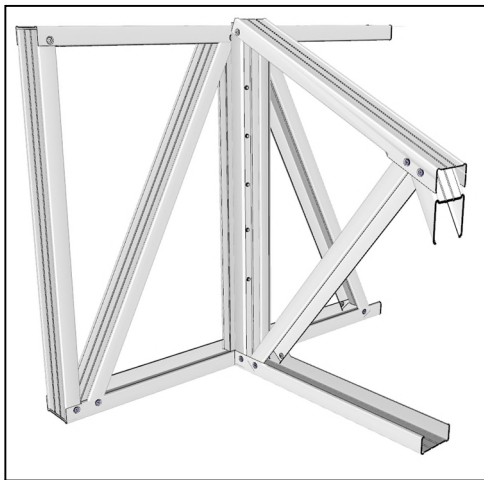
C Section Jack Truss to C Section Girder
