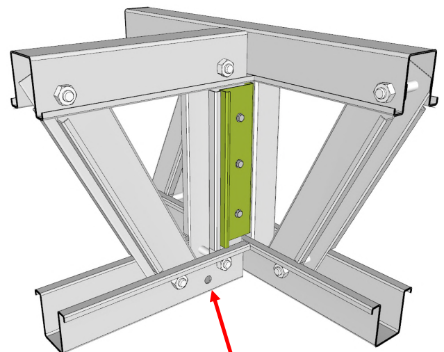
Orientation Hole
