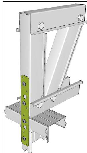
Vertical Strap Hold Down
